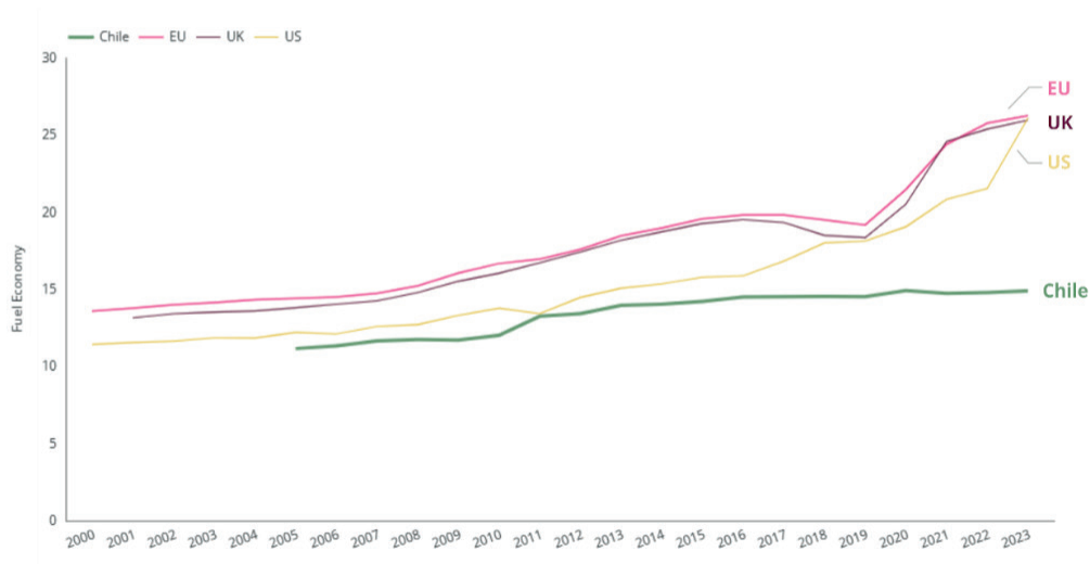
Figure 32. Vehicle performance between the years 2000 and 2023 in the EU, UK, US and Chile, measured in [km/lge].
